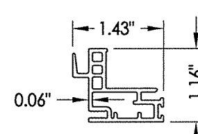
5 MEETING RAIL
