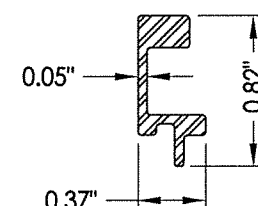
1.4 SASH/STILE & RAIL REINFORCEMENT
