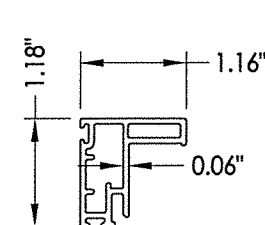
SASH STILE/RAIL
