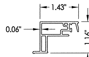
LOCK RAIL
