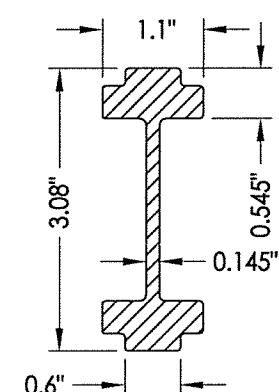
11 MULLION REINFORCEMENT
