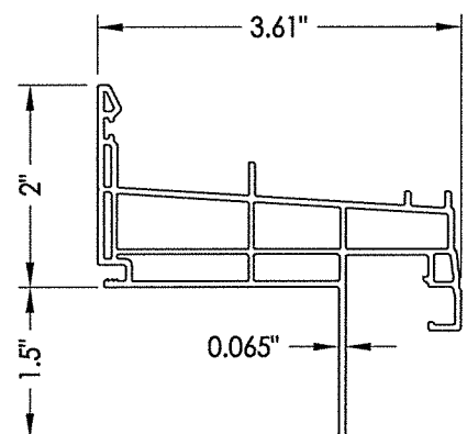
4 SILL
