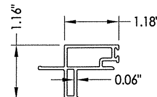
② TOP RAIL
