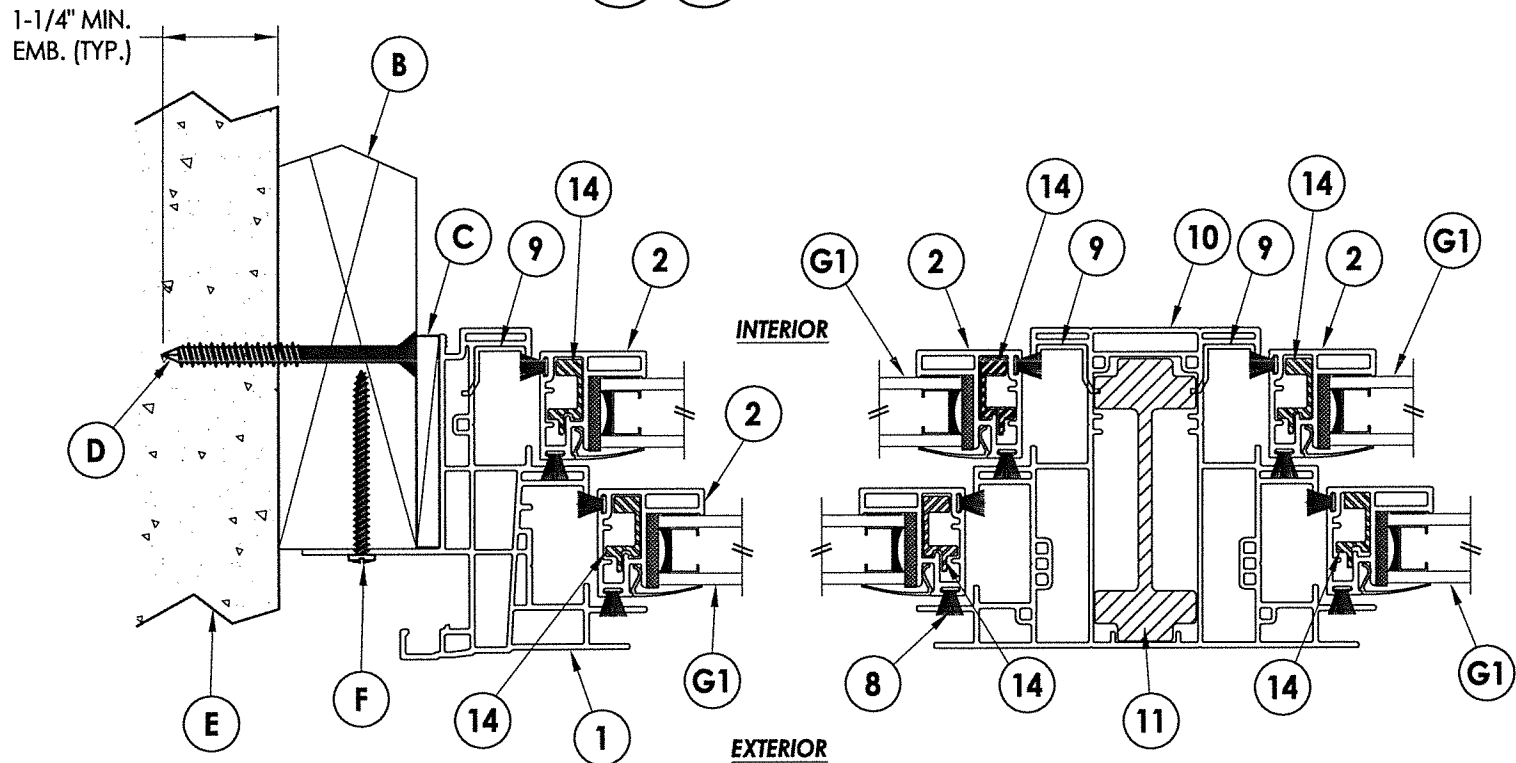
1 HORIZONTAL CROSS SECTION 2 2x Buck Construction
